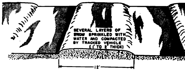
Figure 5-7. Road reinforced with snow.
