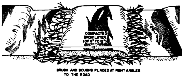
Figure 5-8. Road reinforced with brush and snow.
