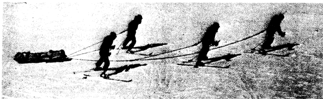
2 Herringbone
